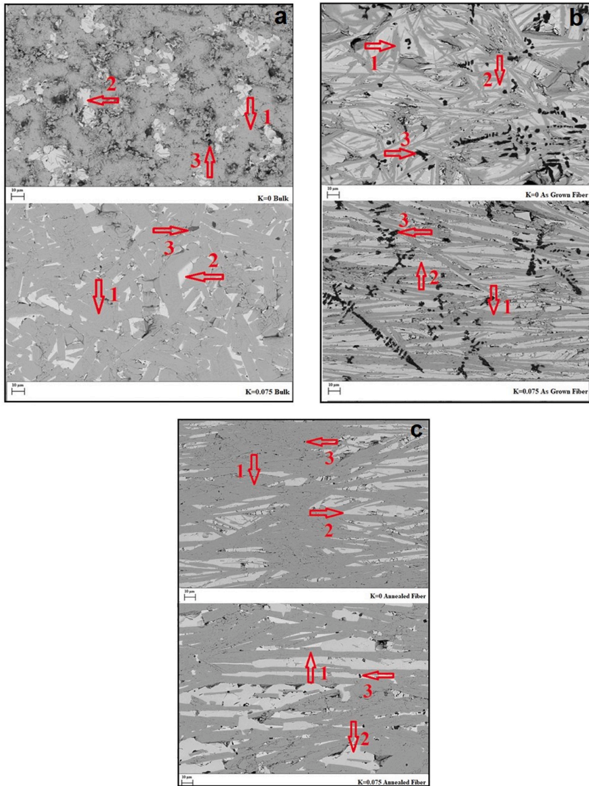
Fig. 2. SEM micrographs and EDS analysis performed in representative \text{BiCa}_{2-x}\text{K}_x\text{Co}_2\text{O}_y samples, (a) bulk; (b) as-grown; and (c) annealed fibers.
