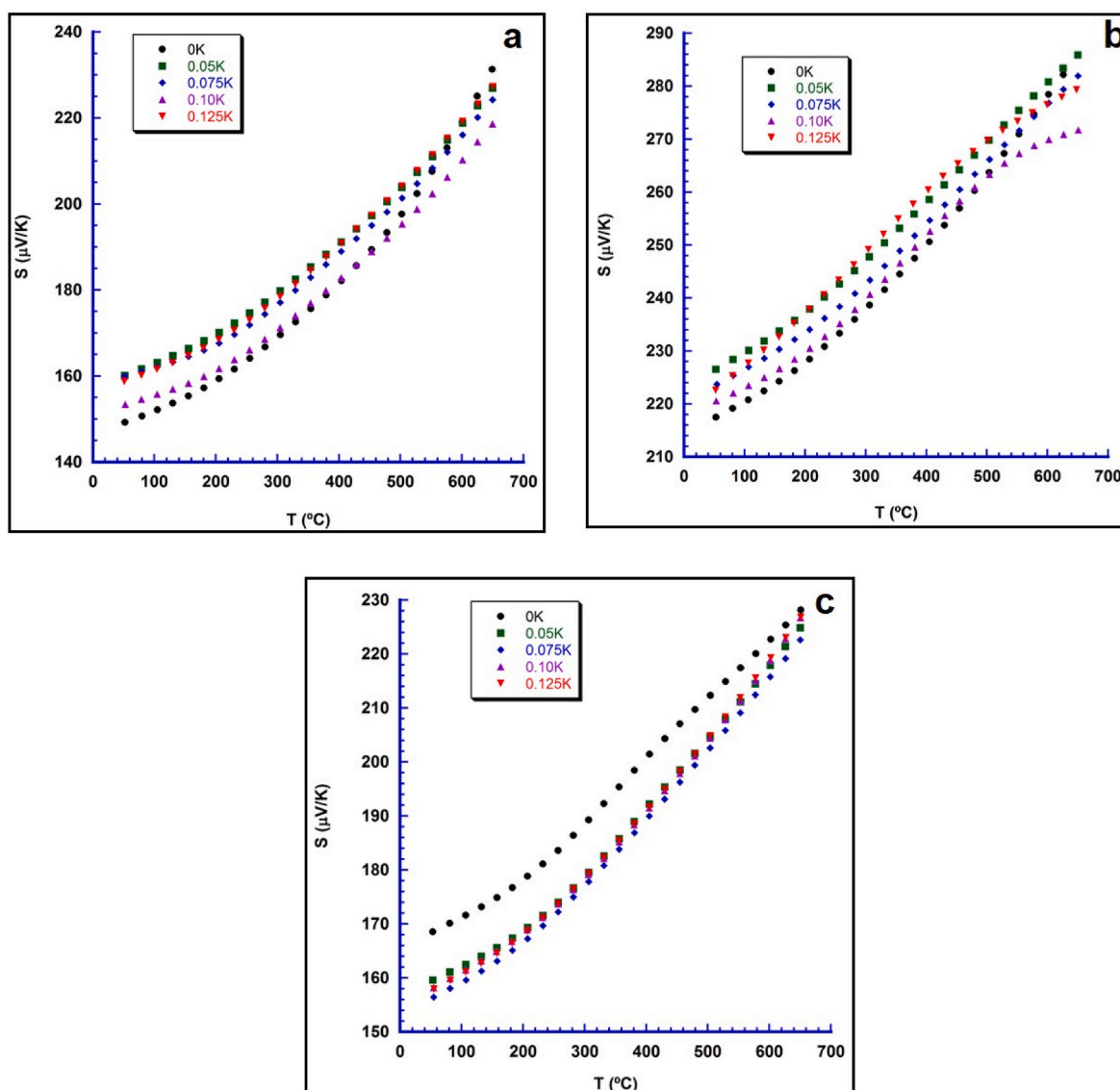
Fig. 5. Seebeck coefficient variation with temperature for all \text{BiCa}_{2-x}\text{K}_x\text{Co}_2\text{O}_y samples, (a) bulk; (b) as-grown; and (c) annealed fibers.
