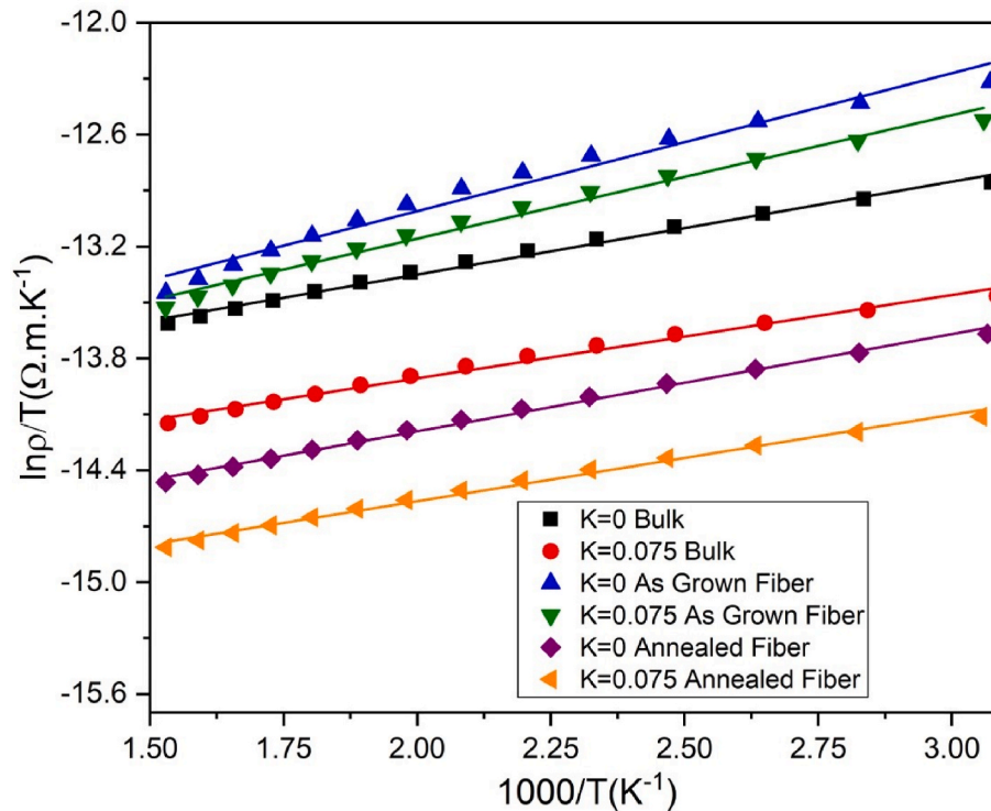
Fig. 4. \ln(\rho/T) versus 1000/T graph of representative \text{BiCa}_{2-x}\text{K}_x\text{Co}_2\text{O}_y samples, for x = 0 and 0.075 .
