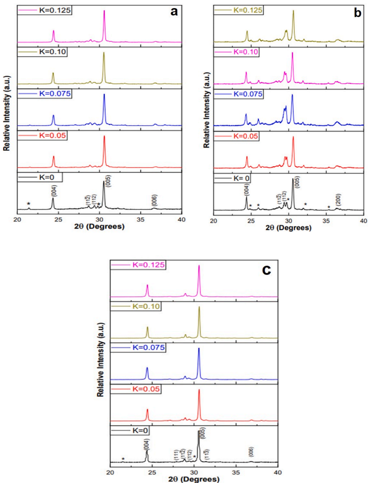
Fig. 1. XRD patterns for all \text{BiCa}_{2-x}\text{K}_x\text{Co}_2\text{O}_y samples, (a) bulk; (b) as-grown; and (c) annealed fibers.
