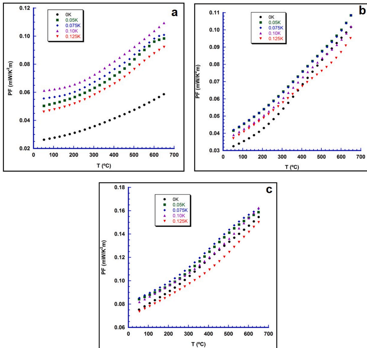
Fig. 6. Power Factor evolution with temperature for all \text{BiCa}_{2-x}\text{K}_x\text{Co}_2\text{O}_y samples, (a) bulk; (b) as-grown; and (c) annealed fibers.
