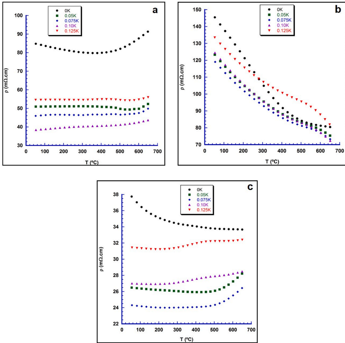
Fig. 3. Electrical resistivity variation with temperature for all \text{BiCa}_{2-x}\text{K}_x\text{Co}_2\text{O}_y samples, (a) bulk; (b) as-grown; and (c) annealed fibers.
